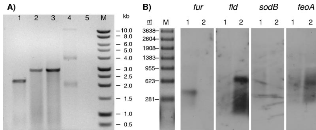
FIG. 2. (A) PCR analysis of Km^r D. vulgaris transformants using primers targeting regions outside of the fur knockout cassette (P7/P8). Lane 1, wild type; lane 2, transformant A; lane 3, transformant B; lane 4, pMO707; lane 5, no DNA; lane M, 1-kb marker. An increase in product size from 2,168 bp to 2,839 bp indicates exchange of the fur gene for the Km^r determinant, creating JW707. (B) Northern analyses of total RNA (10 \mu\text{g} ) from JW707. Lane 1, wild type; lane 2, JW707; lane M, RNA marker. Probes used for hybridization are indicated above the blot. nt, nucleotides.
