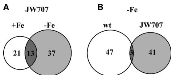
FIG. 5. (A) Genes differentially expressed threefold in the \Delta fur mutant, JW707, compared to wild-type cells, under iron-replete (+Fe; 60 \mu\text{M} ) and iron-limited (-Fe; 5 \mu\text{M} ) conditions. (B) Overlap of genes differentially expressed threefold in JW707 iron-limited (-Fe; 5 \mu\text{M} ) conditions compared with JW707 iron-replete conditions versus those differentially expressed in iron-limited wild-type cells compared to iron-replete wild-type cells.
