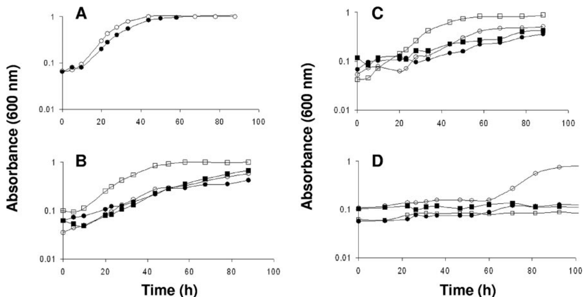
FIG. 3. Growth curves of the D. vulgaris wild type (open symbols) and mutant strain JW707 (filled symbols) under various conditions. (A) Growth under iron-replete conditions ( 30 \mu\text{M FeCl}_2 ). (B) Response to osmolarity stress, with sodium as 300 mM NaCl (circles) or 300 mM NaCl plus 2 mM glycine betaine (squares). (C) Response to osmolarity stress, with potassium as 300 mM KCl (circles) or 300 mM KCl plus 2 mM glycine betaine (squares). (D) Response to nitrite at 2 mM \text{NaNO}_2 (circles) and 5 mM \text{NaNO}_2 (squares). Curves are representative of three trials at 37^\circ\text{C} .
