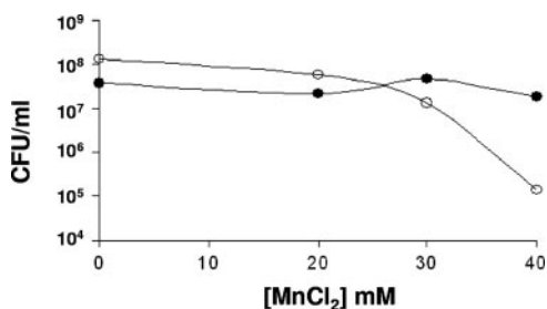
FIG. 4. Growth response of the D. vulgaris wild type (open symbols) and mutant strain JW707 (filled symbols) to \text{MnCl}_2 treatment. Curves are representative of three trials at 37^\circ\text{C} .
