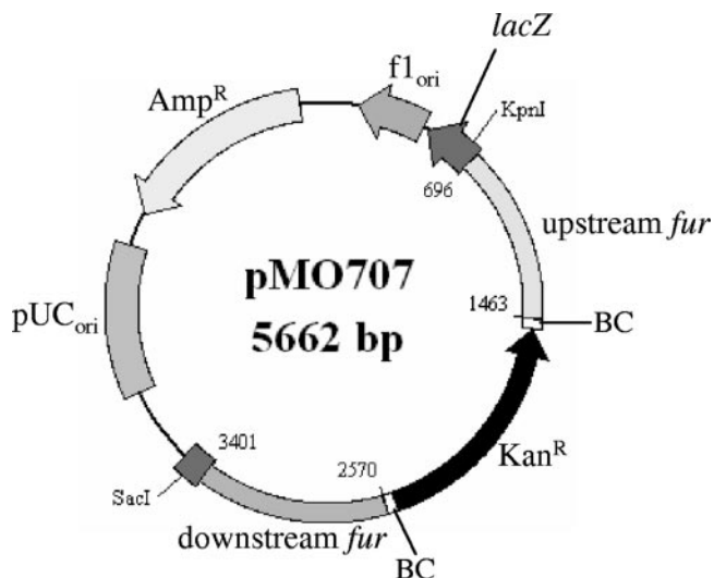
FIG. 1. Map of pMO707 containing the fur deletion construct. A 2,706-bp PCR product containing the pSC27 Km^r determinant flanked by DNA sequences upstream (768 bp) and downstream (831 bp) of the D. vulgaris fur gene was inserted into the EcoRV site of the pBluescript SK(+) multicloning site. Both pBluescript and pMO707 are unstable in D. vulgaris . Numbers indicate positions of sequences upstream and downstream of the fur gene; BC indicates molecular barcodes allowing mutant tracking in a mixed population.
