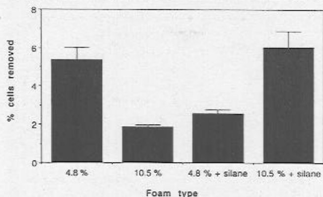
Figure 1 Effect of biomass concentration and silane in the washout of B. cepacia PR131 cells embedded in foam formulations containing the 1% surfactant HS-3. Silane was added at a final concentration of 0.02%. The final biomass concentration (dry wt/wet wt) used was 4.8 or 10.5. Values represent mean percentages of total embedded B. cepacia PR131 cells removed from duplicate columns containing 2 g of foam during passage of 50 ml of filter sterilized water. Error bars indicate standard deviation of means.
