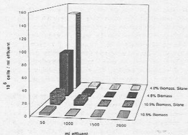
Figure 3 Cumulative washout of embedded B. cepacia PR131 bacteria in foams used in Figure 1. A total of 2 L of water was passed through foam columns. The first 50 ml were collected, followed by 950 ml, 500 ml, and 500 ml. Values represent mean cell density in each sample.
