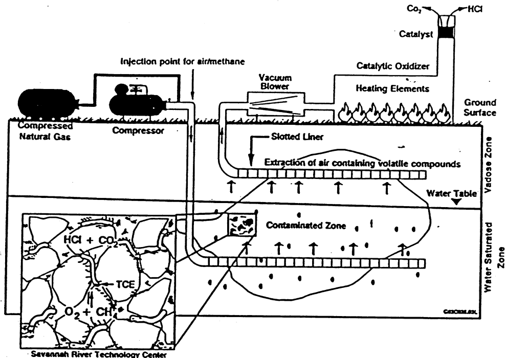
Figure 1. This illustration provides a pictorial view of the horizontal wells in relation to the surface mounted equipment.
