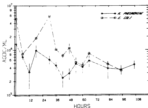
Fig. 3. Changes of in situ densities of Klebsiella pneumoniae and Escherichia coli by AODC over time (mean ± 1 standard error).
