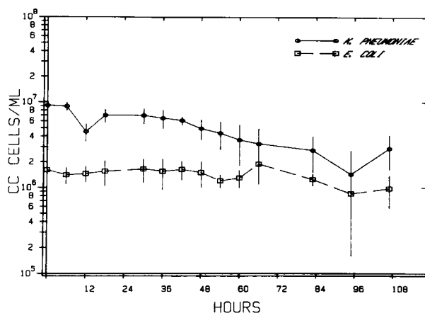
Fig. 2. Changes of in situ densities of Klebsiella pneumoniae and Escherichia coli by Coulter counter over time (mean \pm 1 standard error).
